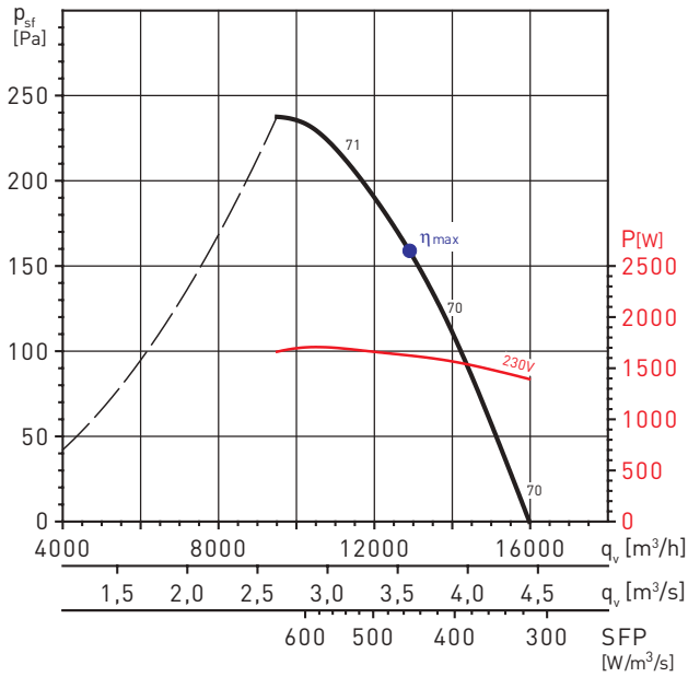
TCBB/4-630/L
