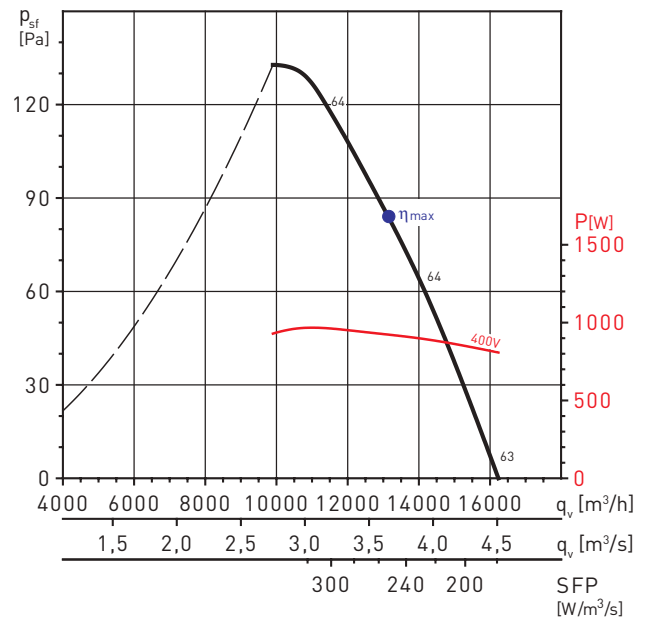
TCBT/6-710/L
