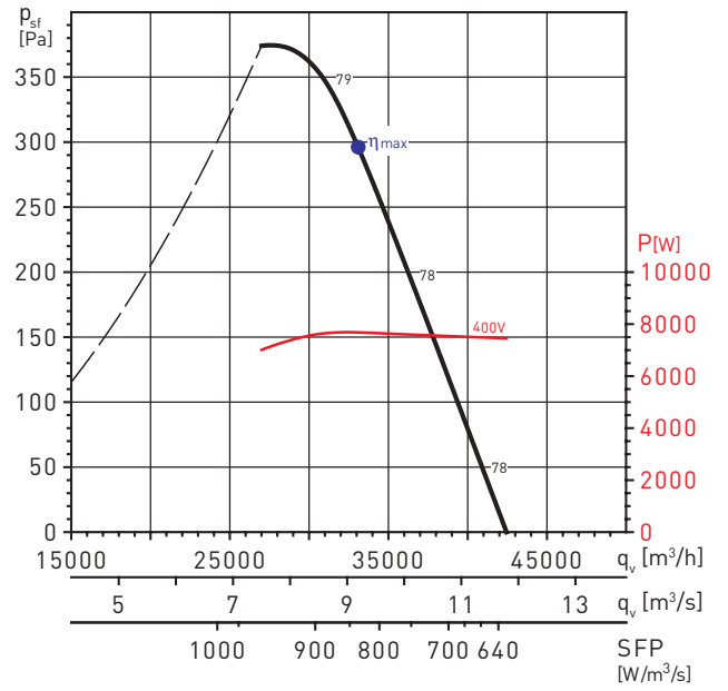
TCBT/4-800/H
