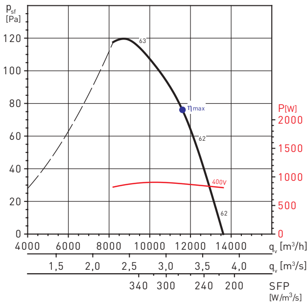
TCBT/6-630/H
